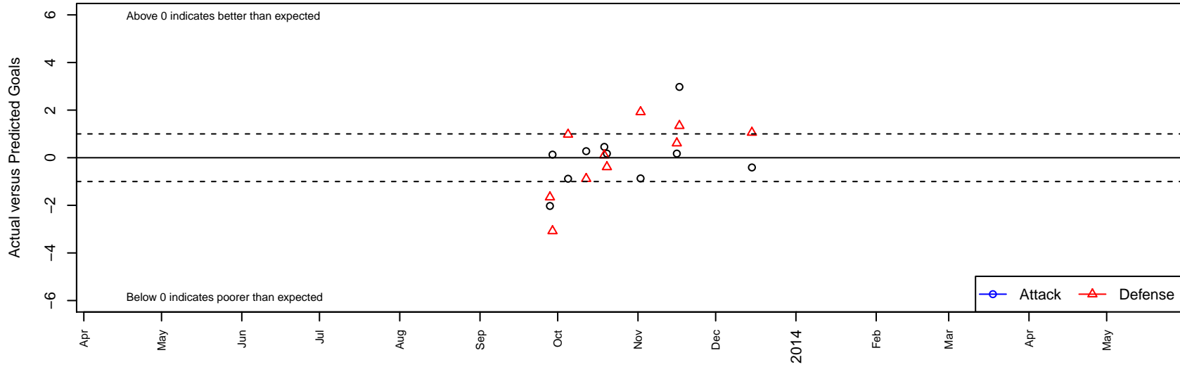
Impact SC B02 Dots are actual minus expected GF (blue circles) and GA (red triangles). Blue line is smoothed change in attack strength. Red is smoothed change in defense strength.
